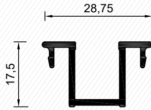
Tek Cam Adaptör Profili - Adapter Profile
